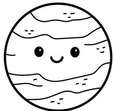
NEPTUNE
