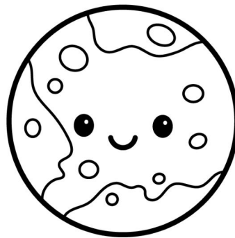
MERCURY
