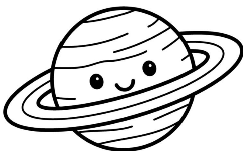
SATURN
